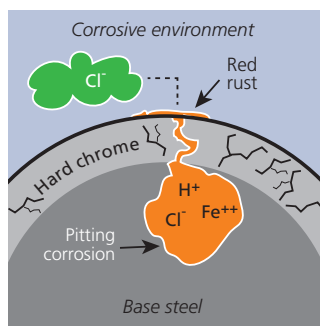
Corrosion mechanism of hard chrome plated bar
