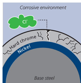
Barrier protection of the inner nickel layer
