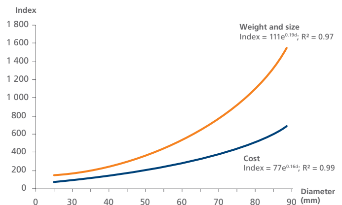
Cost and weight development of a piston rod
